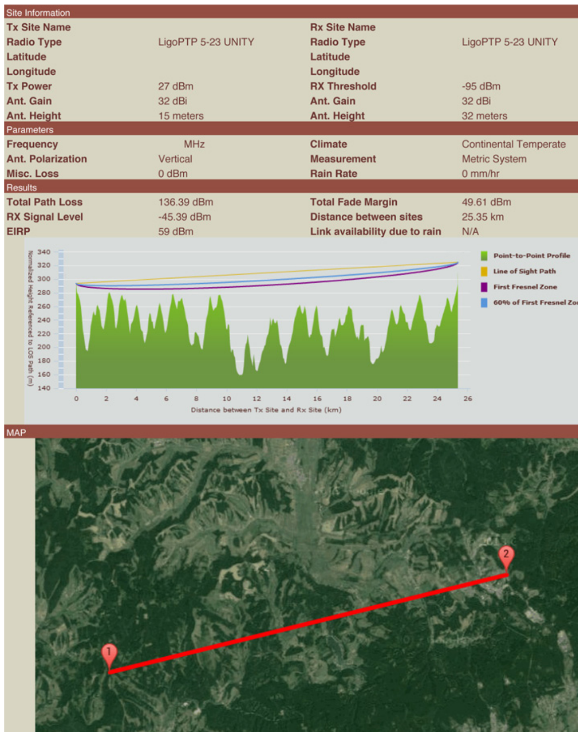
Picture 1: Link path analysis and satellite map illustration
